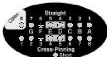
Open Pair Straight open wire #3 Cross-pinning open wire #6
